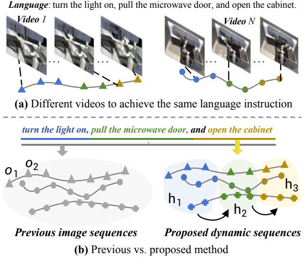
Figure 1. (a) The mismatch between the simplicity and singularity of language and the diversity and complexity of videos. (b) Instead of directly mapping language to video content, DynaMind bridges this gap by abstracting video into dynamic representations, enabling high-level dynamic reasoning for decision-making.
