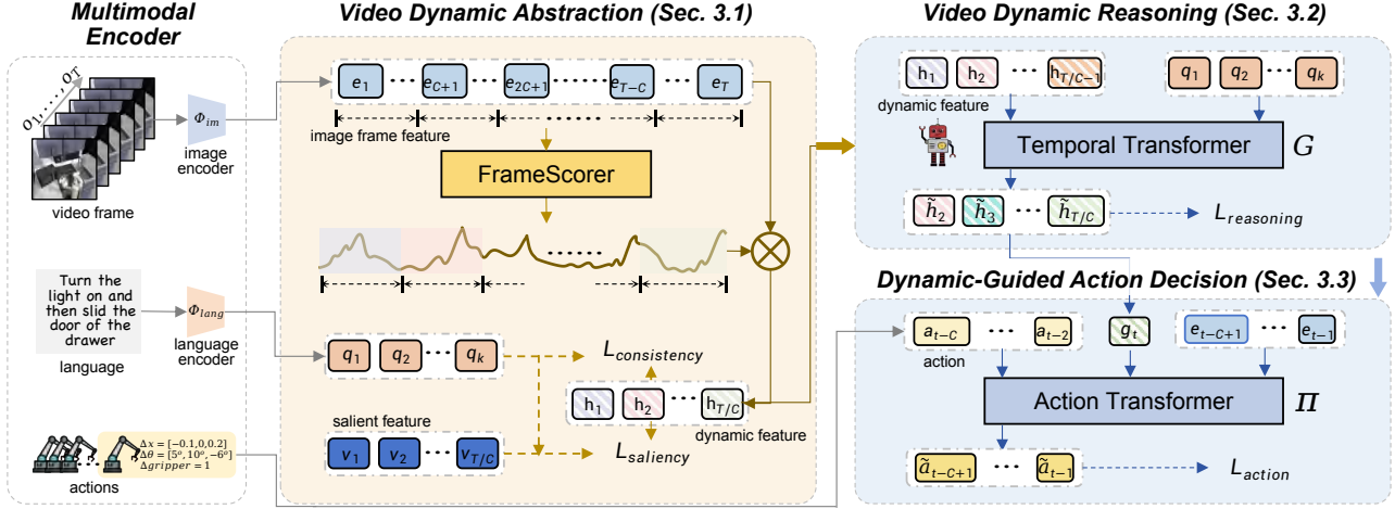
Figure 2. Overview framework of DynaMind. DynaMind begins with Video Dynamic Abstraction , which converts video into dynamic representations. Then, Video Dynamic Reasoning predicts future dynamics. Finally, Dynamic-Guided Action Decision uses the predicted dynamics to infer the corresponding action sequence. These modules are integrated for shared feature encoding, enabling end-to-end training. During training, future frames and actions serve as supervision, while inference relies solely on historical information.
