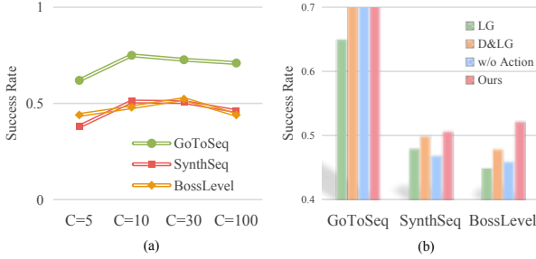
Figure 7. (a) Ablation on dynamic reasoning. (b) Ablation on dynamic-guided action decision.
