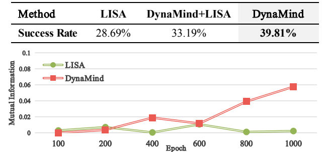
Figure 8. Top: Results of the combined method. Bottom: Mutual information over training.
