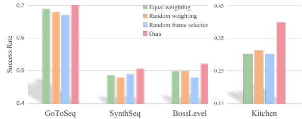
Figure 6. Ablation on dynamic abstraction.
