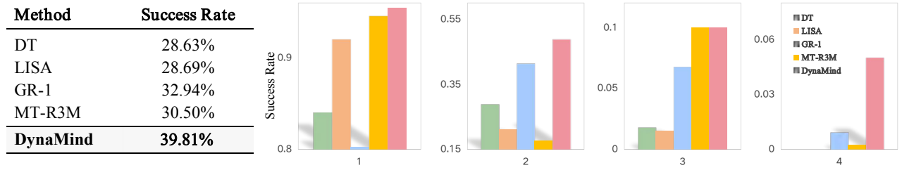
Figure 3. Success rates on Franka Kitchen. The four plots on the right illustrate the success rates of completing 1 to 4 subtasks within a single episode, while the left plot shows the average success rate across all tasks. The evaluation is repeated 100 times.
